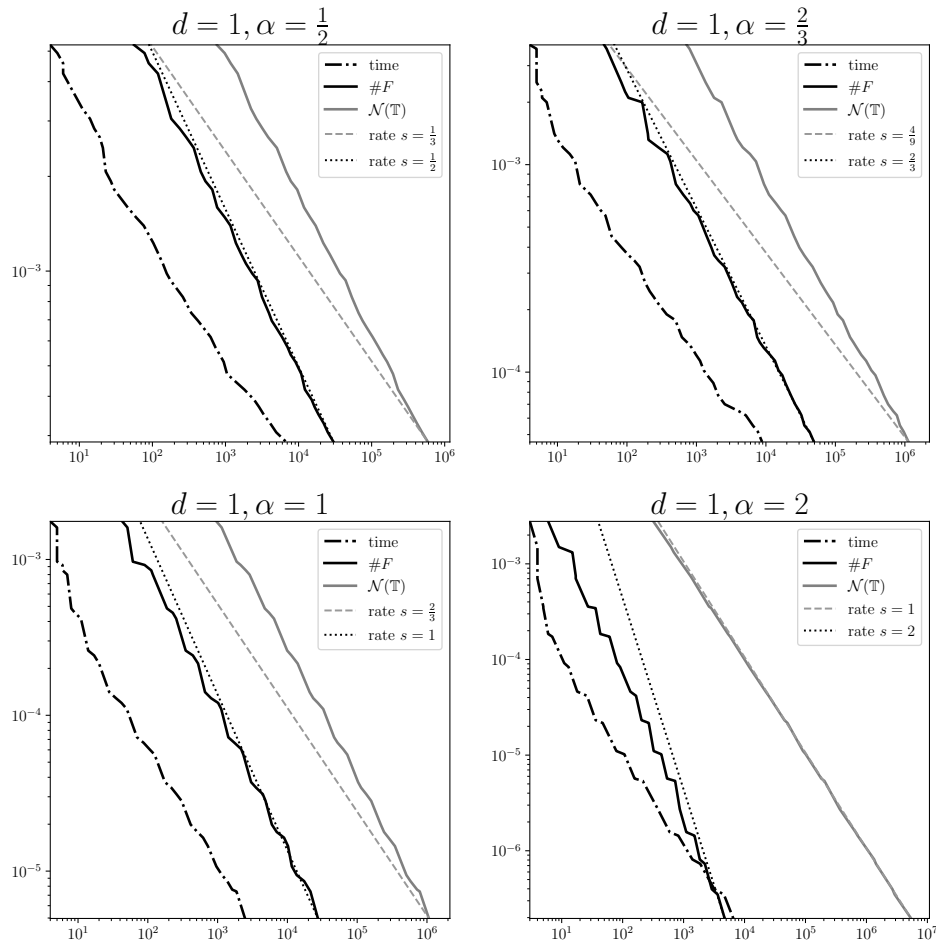
Figure 3: Computed residual bounds for d = 1 as a function of degrees of freedom \dim \mathcal{V}(\mathbb{T}) \approx N(\mathbb{T}) of the current approximation of u (solid grey lines), degrees of stochastic freedom \#F (solid black lines), and elapsed computation time in seconds (dash-dotted line).
