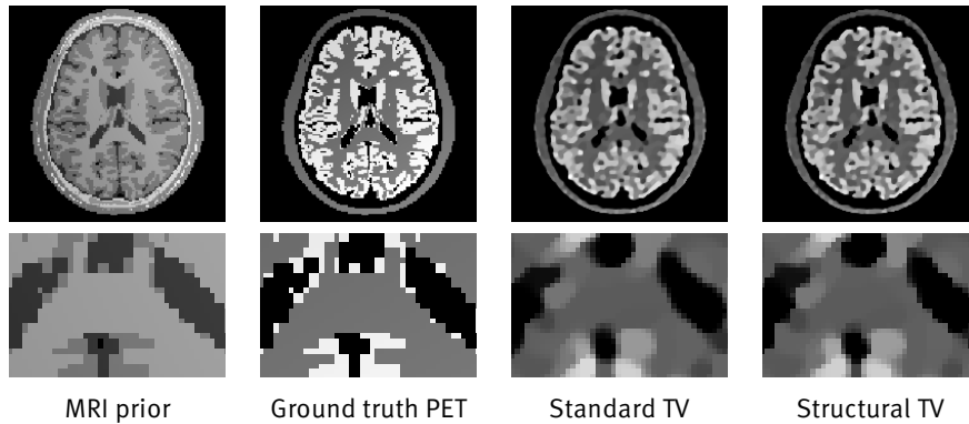
Fig. 1: Better reconstruction of the edges of a PET image using an MRI image as structural prior
