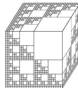
Fig. 5: Cantor set of order 5 as model for geological network of faults and cracks
