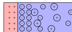
Fig. 1: Accumulation of negative ions at positively charged electrode surface
