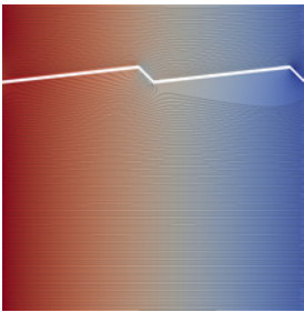
Fig. 5: Solution to the Stokes-Darcy coupled problem for a "river bed" computed by PARMOON
