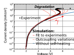
Fig. 4: Simulated S-shaped current-voltage relations for different thermal outcoupling
